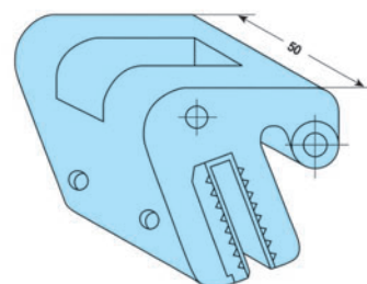
D PINZA D CLAMP
