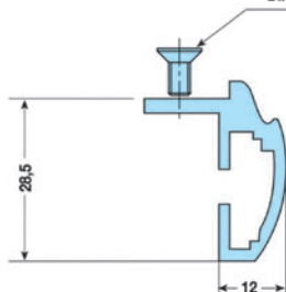
PERFIL CARTELA FRONT TRIM PROFILE
