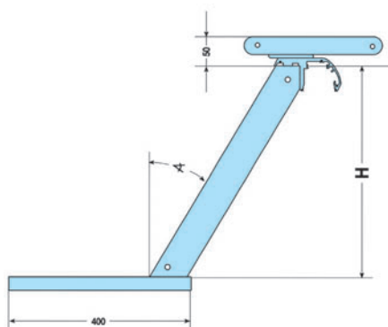
MONTANTE CB1 HOLDER CB1
