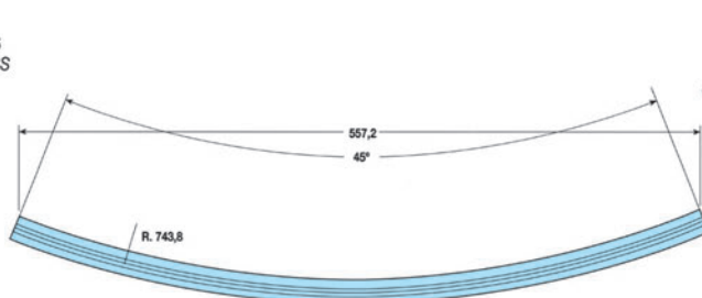
PERFIL TIRADOR COMPLETO CURVO INTERIOR, BBS INTERNAL CURVED COMPLETE HANDLE PROFILE, BBS
